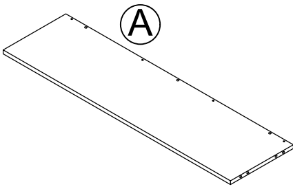
TOP T4865837010GO QTY: 1 PC
